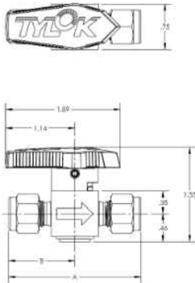
P4 Series
