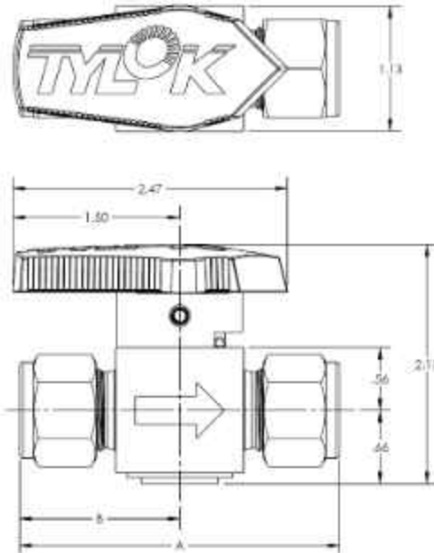
P6 Series
