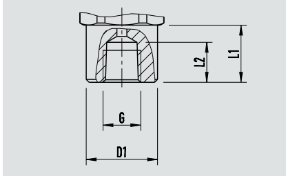
ANSI/ASME B1.20.1, female thread
