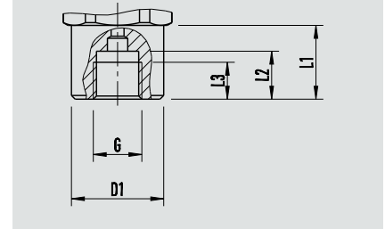
EN 837, female thread
