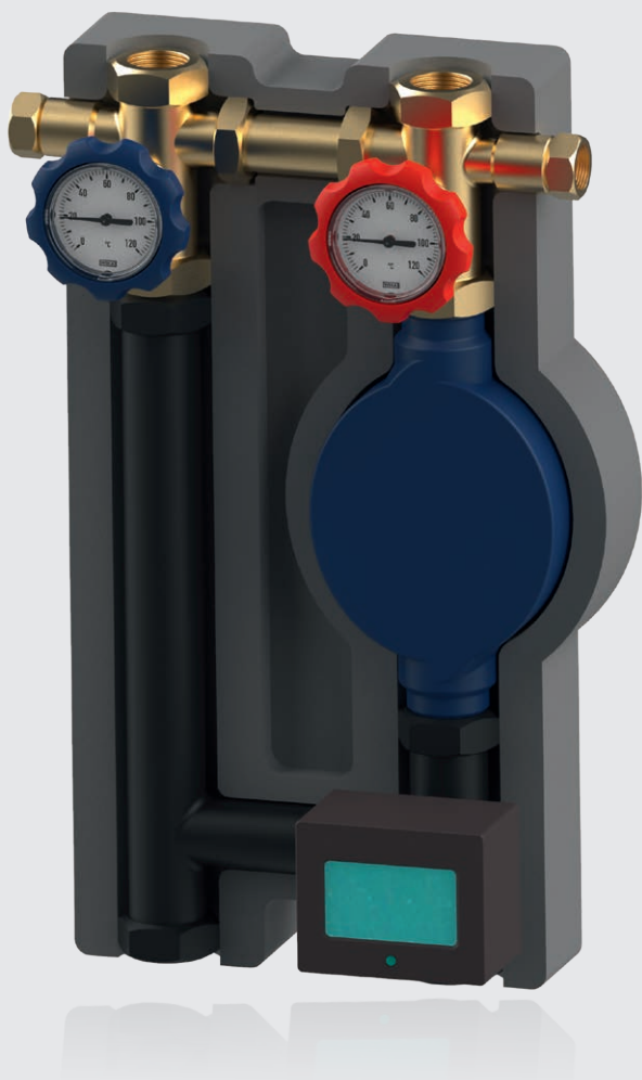
Pump assembly with two WIKA thermometers
