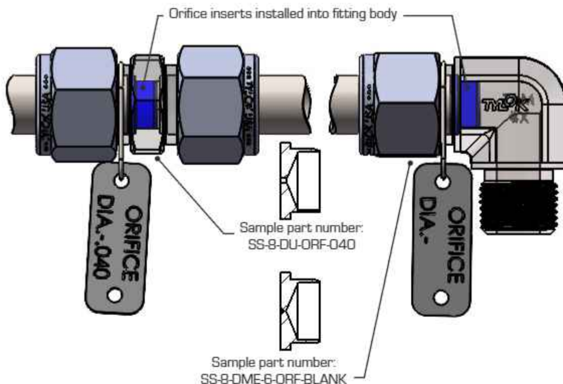
Four ways to order Orifice Inserts for CBC Tube End Sizes 4 (1/4") through size 16 (1")
