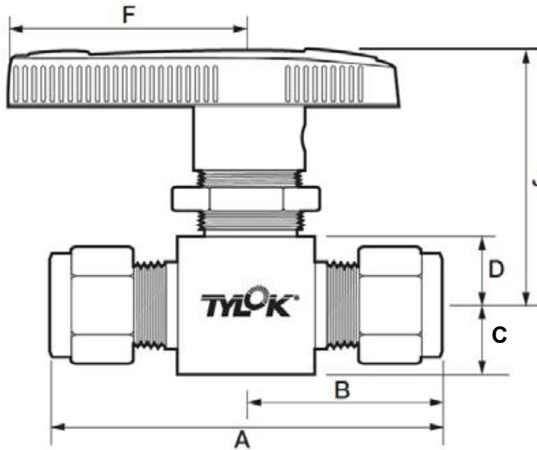
Straight Ball Valve
