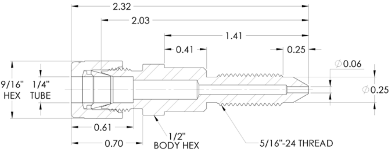
Fits Tylok Bleed Valves
