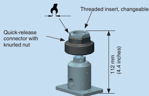
2,500 bar (36,250 psi) measuring instrument stand
