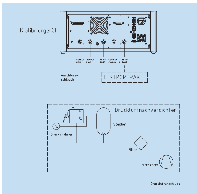
Connection diagram for pressure supply package, Model CPK-PS40, P_{\max} = 40 bar (580 psi)
