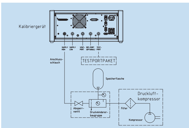
Connection diagram for pressure supply package, model CPK-PS300, P_{\max} = 250 bar (3,625 psi)
